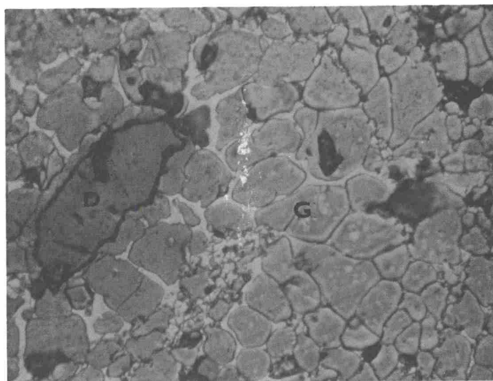
Fig. 15.--Polished High Pressure Orthorhombic GdSb_2 500X
